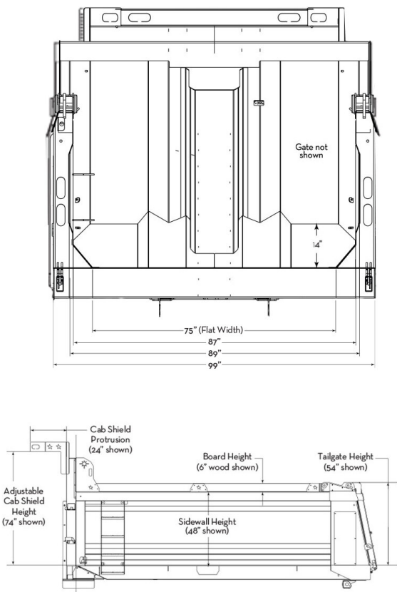
Representative dimensional drawing. Sidewall, board, tailgate and cab-shield heights shown are one configuration — yours is built to order.
